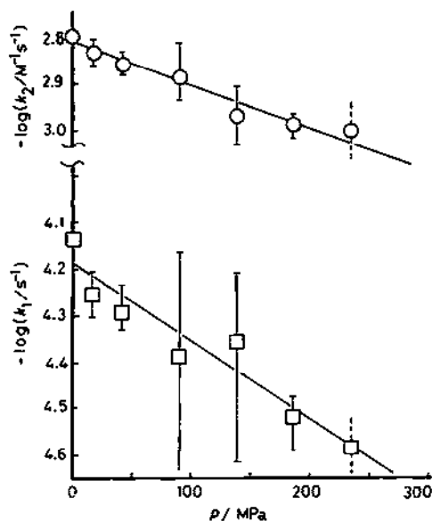
Fig. 3. Pressure dependence of k_1 and k_2 for the ligand isotopic exchange of [\text{Al}(\text{acac})_3] in acetylacetone at 25^\circ\text{C} : \square , k_1 ; \circ , k_2 .
