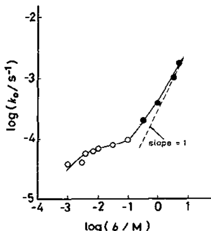
Fig. 5. Log-log plot of the observed isotopic exchange rate constant k_0 of [\text{Cr}(\text{acac})_3] vs. the concentration of free ligand ( b ) in acetonitrile at 166°C: [\text{H}_2\text{O}] = 0.70 \pm 0.005 \text{ M} .
