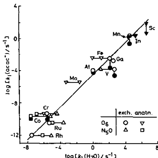
Fig. 6. The linear free energy relationship between ligand isotopic exchange rates of [M(III)(acac)_3] and aqua complexes of M(III) at 25^\circ C . Ordinate, k_1 for [M(acac)_3] : \circ , \Delta , \nabla , \square , in Hacac; \nabla , in mixed solvent; \bullet , \nabla , \blacksquare , in acetonitrile. Abscissa: first-order rate constants for water exchange ( \circ ) and anation ( \nabla ) of [M(H_2O)_6]^{3+} , and water exchange ( \Delta ) and anation ( \square ) of [M(NH_3)_5(H_2O)]^{3+} in acid aqueous solution.
